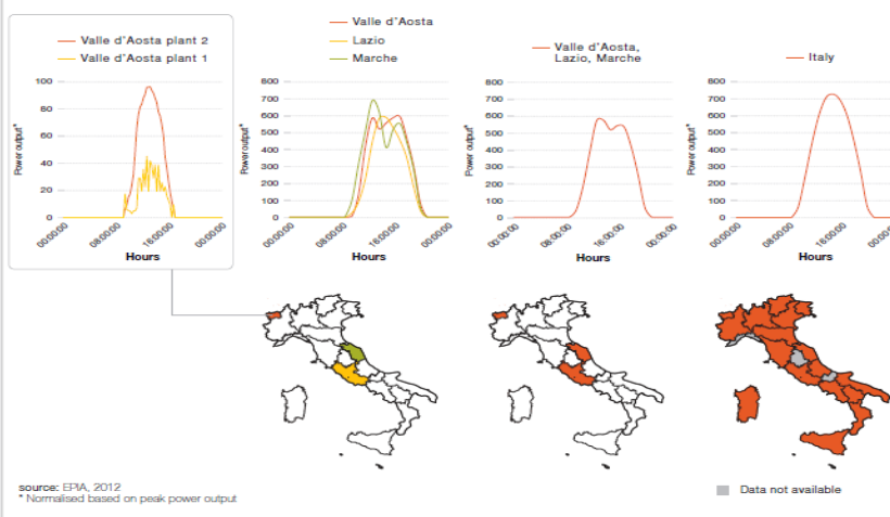
Figure 3 - Comparison of daily PV variability (plant, region and country level) - Example of Italy (kW)
