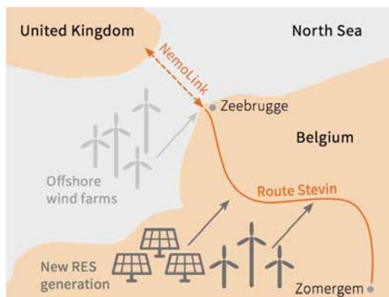
Fig 5 Diagram of the planned Nemo Link and Stevin project connection. Source: National Grid
